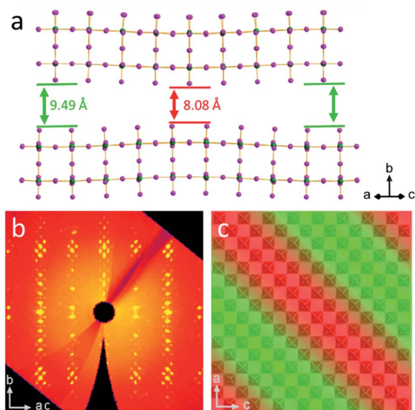
Fig. 2 (a) The modulated IAA n = 2 structure viewed along the (1 0 1) axis showing a single wave in the structure. The minimum and maximum interlayer distances are labeled in red and green, respectively. (b) The diffraction of a single crystal showing the supercell reflections. (c) A view of the crystal structure looking perpendicular to a single layer. The areas colored in green indicate maximum interlayer spacing between two arbitrary layers, and red indicates minimum interlayer spacing.
