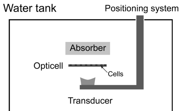
Figure 1. HIFU exposure setup. Our in-house built HIFU apparatus consisting of a motorized transducer, capable of movement in the x, y, and z planes, and a holder for the Opticell™ chamber submerged in a tank of degassed 37°C water. The walls of the tank and the area above the transducer and Opticell™ chamber were lined with an absorptive material, to prevent reflection of the acoustic beam and resulting standing wave formation.
