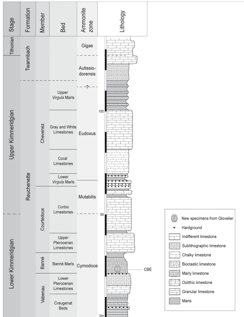
Fig 1. Stratigraphical column of the Reuchenette Formation in northwestern Switzerland. The shell marks the position of the new specimens in the Banné Marls (CBE: Combe du Bé, name of the locality). Modified from Püntener et al. [11].
