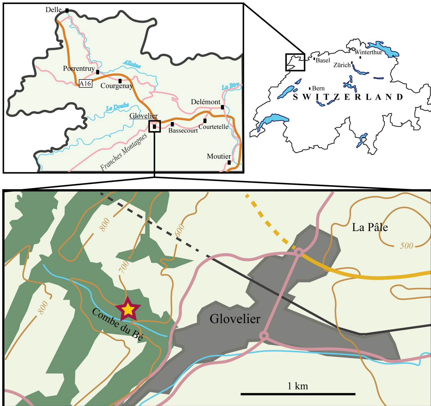
Fig 2. Map of the locality. The star marks the location of the outcrop in the small valley Combe du Bé near Glovelier, Canton of Jura, northwestern Switzerland.
