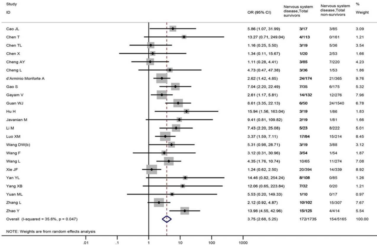
Fig. 3. Association between nervous system diseases and the mortality of COVID-19.
