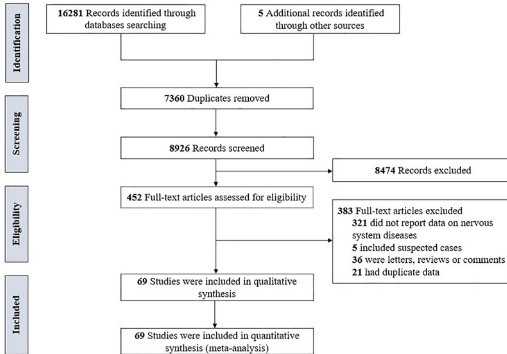
Fig. 1. The flowchart of the screening process.
