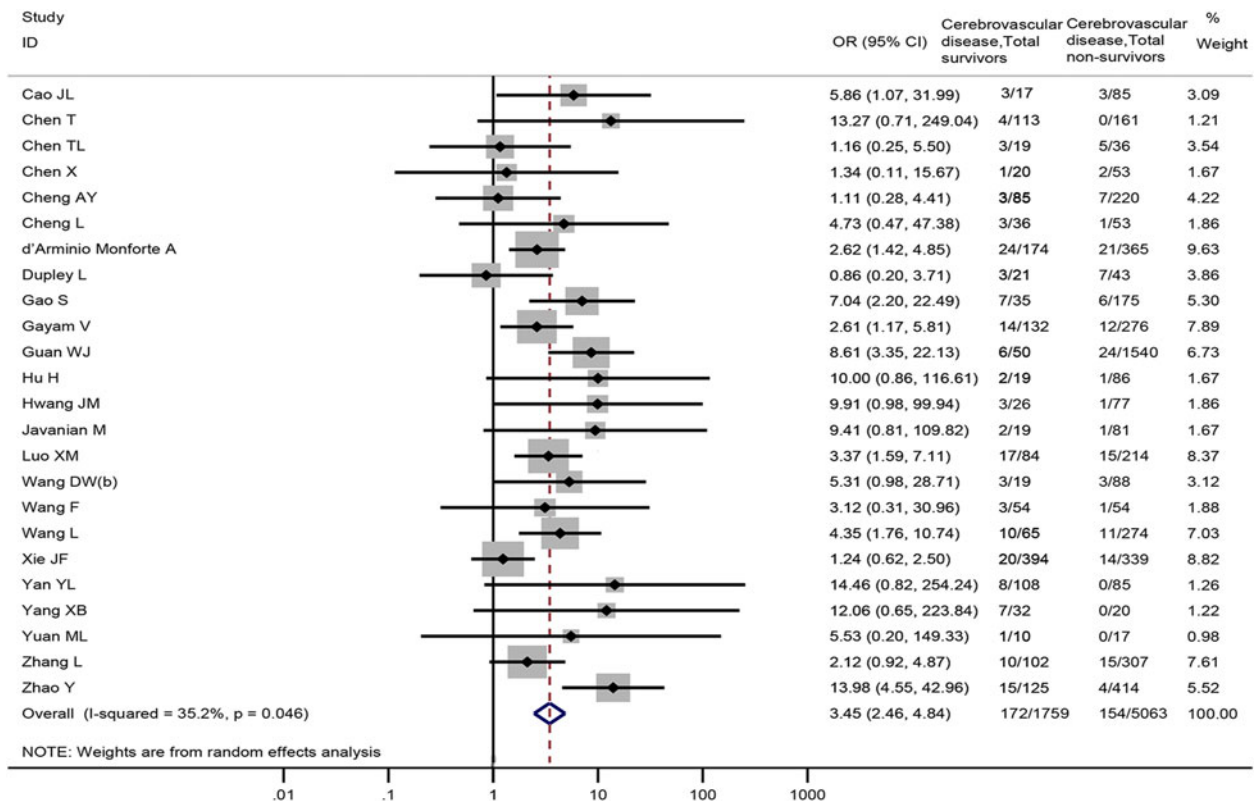
Fig. 5. Association between cerebrovascular disease and the mortality of COVID-19.
