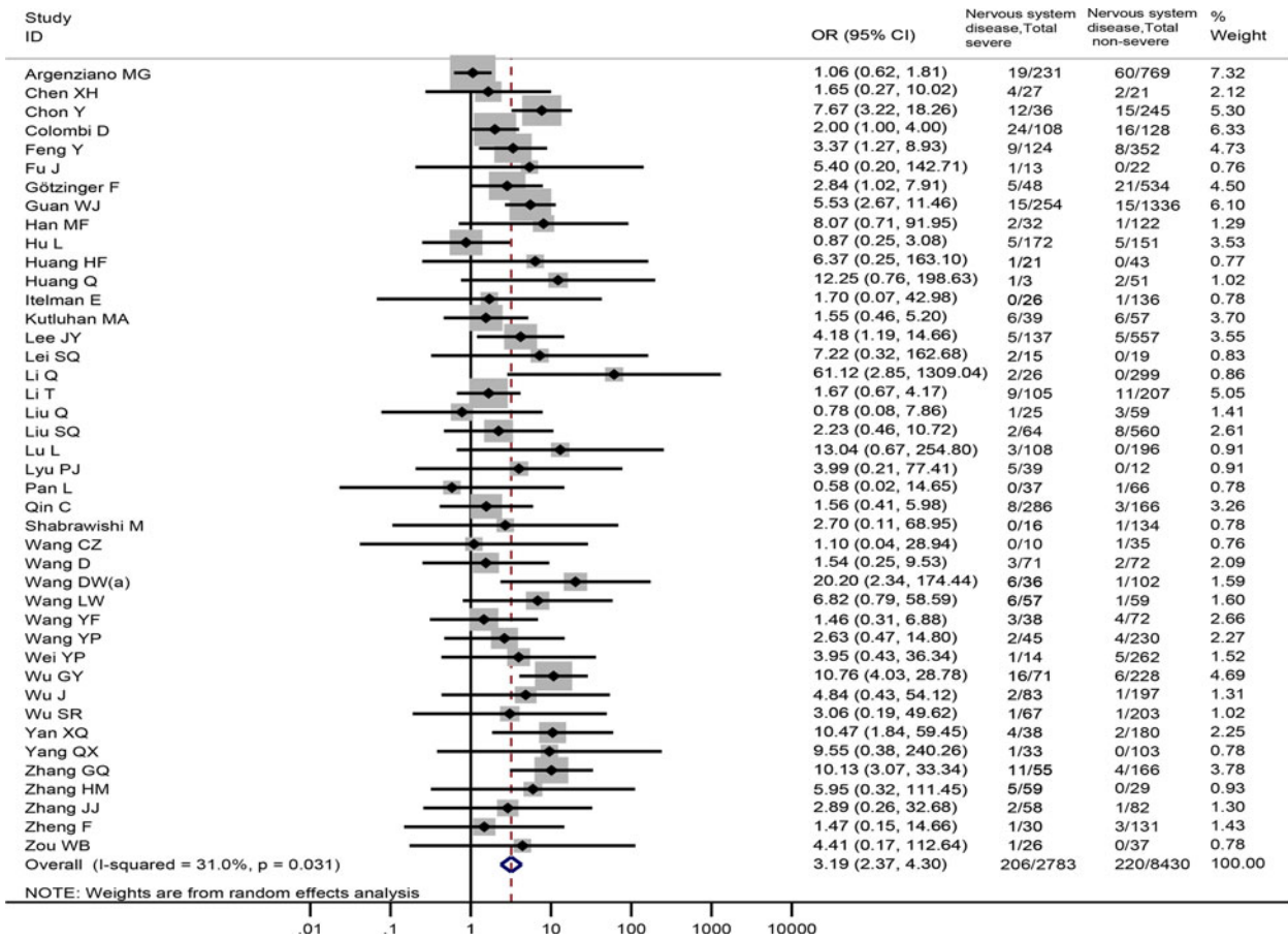
Fig. 2. Association between nervous system diseases and the severity of COVID-19.
