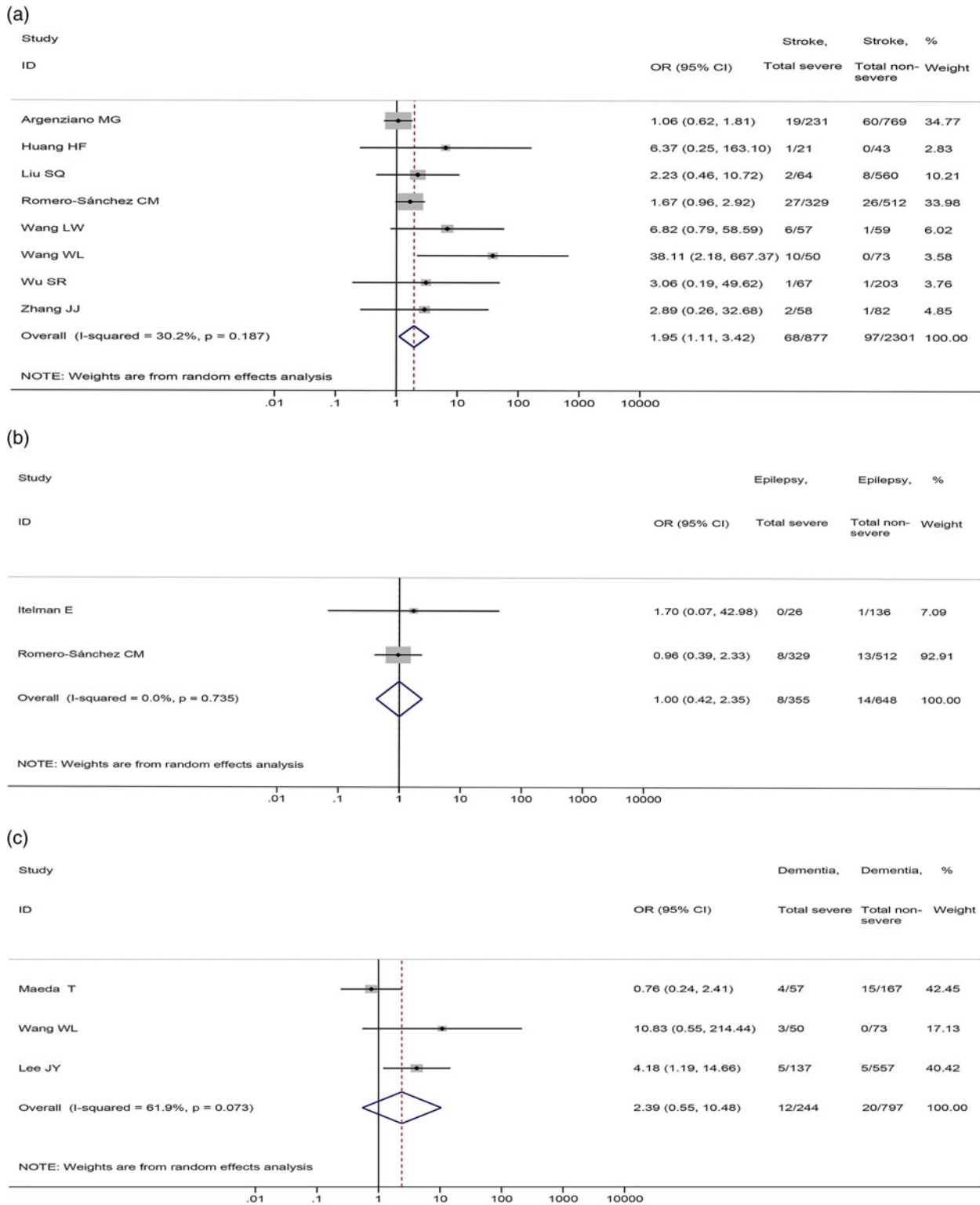
Fig. 6. Association between (a) stroke, (b) epilepsy, (c) dementia and the severity of COVID-19.
