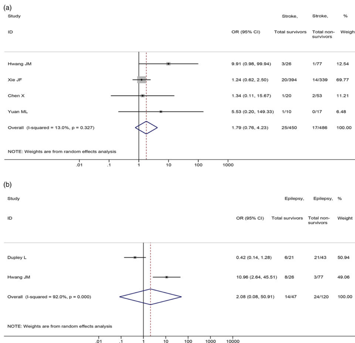
Fig. 7. Association between (a) stroke and (b) epilepsy and the mortality of COVID-19.
