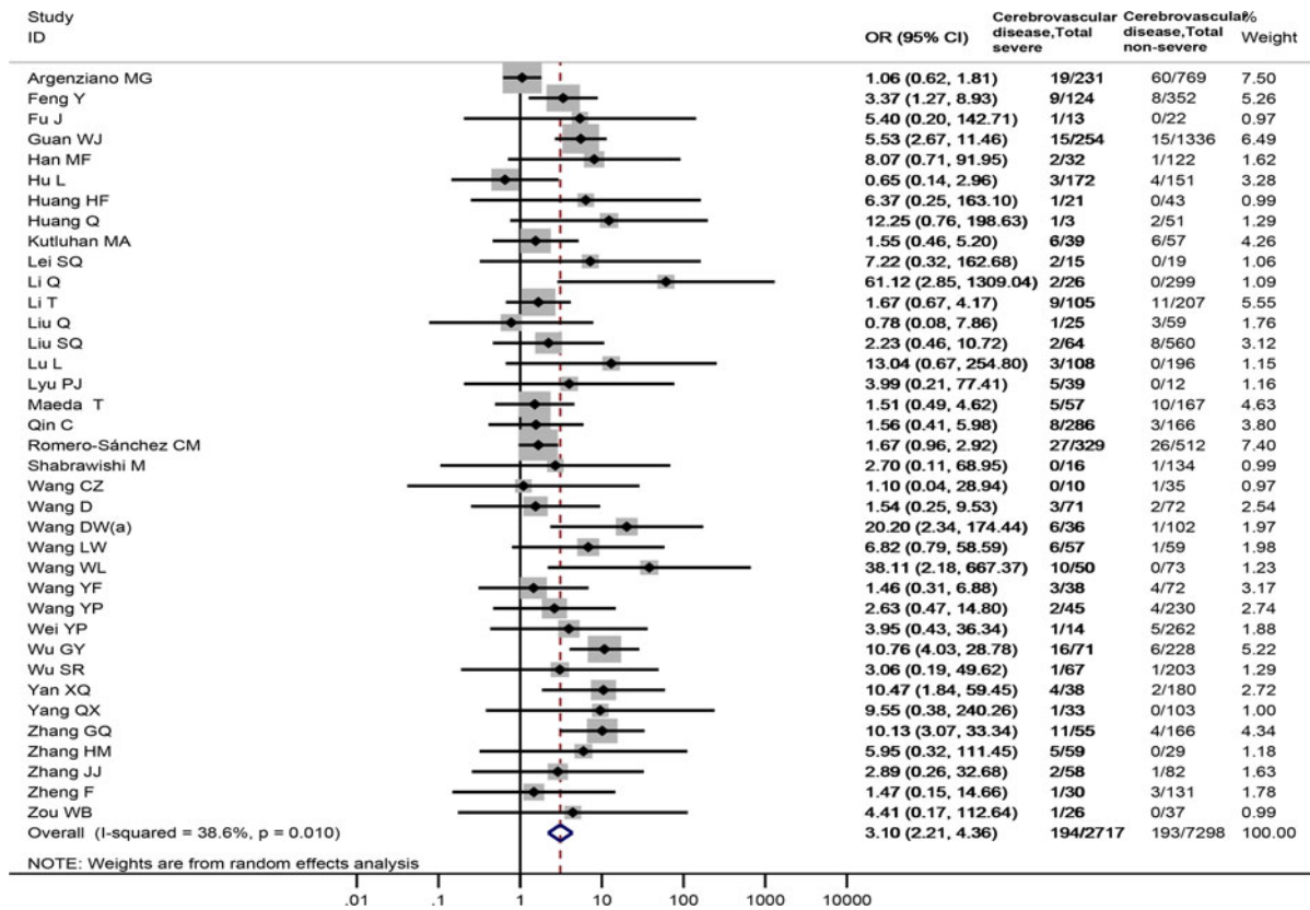
Fig. 4. Association between cerebrovascular disease and the severity of COVID-19.
