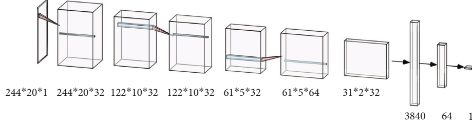
FIGURE 3: CNN structure.
