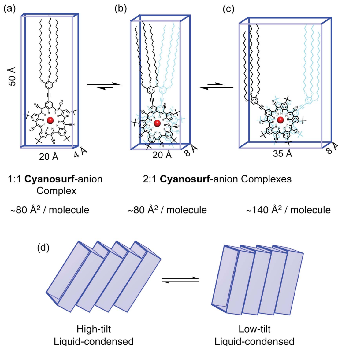
Fig. 6 Molecular models of the supra-amphiphile complexes at the air–water interface as (a) a 1 : 1 complex, (b) 2 : 1 complexes with either \sim 36^\circ or (c) \sim 108^\circ rotation angles that are defined by the sterically-gated tert -butyl groups on the macrocycles. (d) Tilted arrangements of the supra-amphiphiles.
