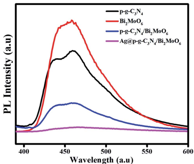
Fig. 8 PL spectra of p-g- \text{C}_3\text{N}_4 , \text{Bi}_2\text{MoO}_6 , p-g- \text{C}_3\text{N}_4/\text{Bi}_2\text{MoO}_6 , and \text{Ag@p-g-C}_3\text{N}_4/\text{Bi}_2\text{MoO}_6 .
