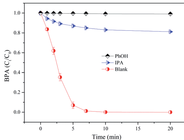
Fig. 8 The effects of IPA and PhOH on BPA degradation in nZVI/SPC system. General reaction conditions: [BPA]_0 = 0.1 \text{ mM} , [nZVI]_0 = 0.1 \text{ g L}^{-1} , [SPC]_0 = 3 \text{ mM} , \text{pH}_0 = 4.0 .
