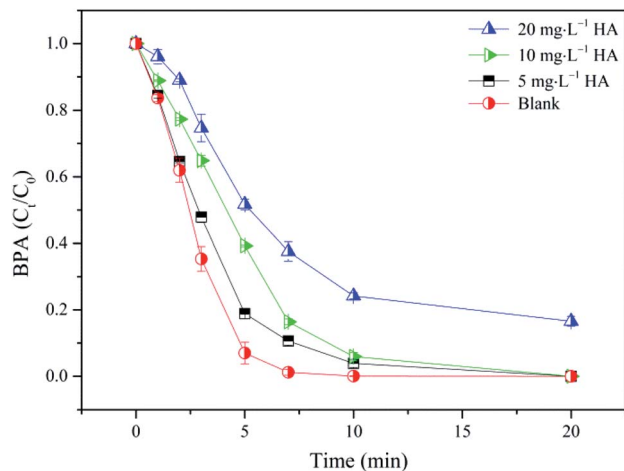
Fig. 7 Effect of HA on BPA degradation in the nZVI/SPC system: [BPA]_0 = 0.1 \text{ mM} , [nZVI]_0 = 0.1 \text{ g L}^{-1} , [SPC]_0 = 3 \text{ mM} , \text{pH}_0 = 4.0 .
