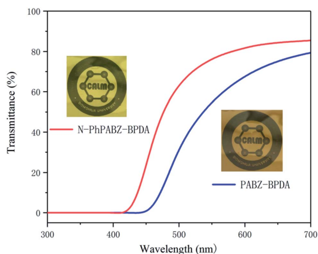
Fig. 5 UV-vis spectra and images of the PBII films.
