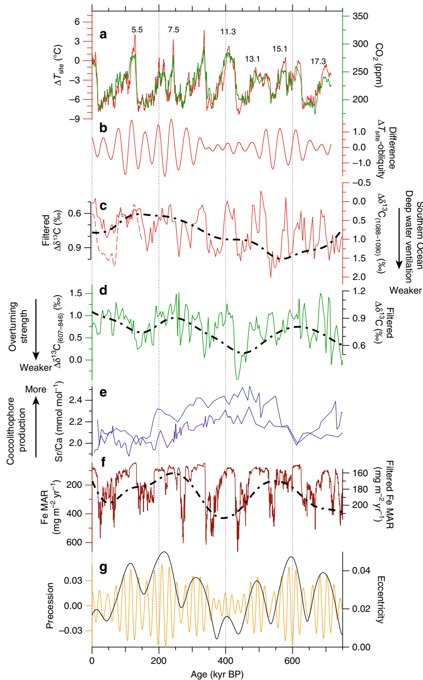
Fig. 5 Link between the 400-kyr phase modulation and the global ocean carbon cycle. a DF \Delta T_{site} (red) and the composite atmospheric CO_2 record 32 (green). b The difference between the normalized obliquity component of \Delta T_{site} and AMI (same as in Fig. 4g). c The intermediate-to-deep \delta^{13}C gradient of benthic foraminifera ( \Delta\delta^{13}C ), a proxy for deep-water ventilation in the Southern Ocean 49 . \Delta\delta^{13}C represents the difference in \delta^{13}C between two cores, specifically those collected at ODP site 1088 (ca. 2100 m water depth) and site 1090 (ca. 3702 m water depth) in the South Atlantic Ocean. Dotted red line indicates the \Delta\delta^{13}C obtained using C. kullenbergi data at site 1090 and solid red line indicates C. wuellerstorfi data only. d A measure of overturning strength based on \delta^{13}C gradient 50 between the North Atlantic (ODP site 607) 91 and the tropical Pacific Ocean (ODP site 846) 92 . Small gradients (close to zero) imply drastically reduced ventilation of the Atlantic or enhanced ventilation in the Pacific 50 . e Sr/Ca of coccolithophores as a proxy for the rate of coccolithophore production in southwestern Indian Ocean (purple line, MD962077) and in the western equatorial Pacific (blue line, V28-239) 45 . f Mass accumulation rate (MAR) of iron in the subantarctic Atlantic Ocean (ODP site 1090) 48 . Dashed-dotted black line indicates the long-term trend obtained using a Gaussian filter around 0 kyr^{-1} with a 0.0045 kyr^{-1} bandwidth (i.e. with periodicity < 222 kyr removed). g Orbital eccentricity (black) and precession (yellow)
