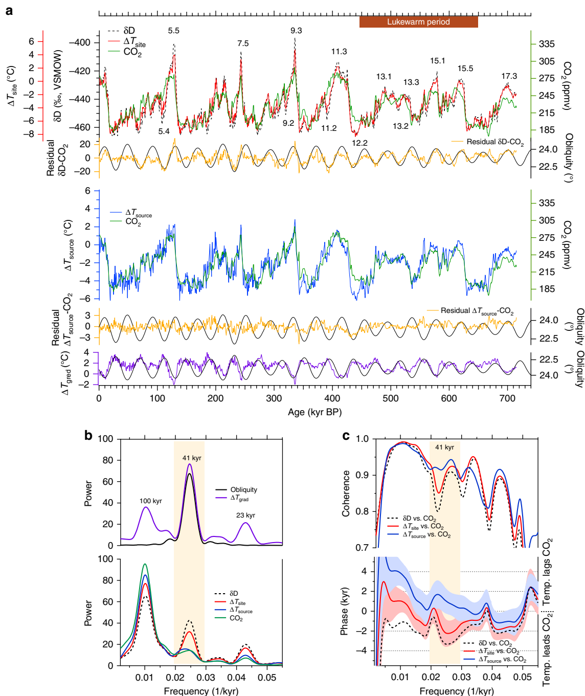
Fig. 3 Temperature reconstructions from the DF2 core together with the \text{CO}_2 record. a The upper panel shows the DF \delta\text{D} (black) and \Delta T_{\text{site}} (red) records and the \text{CO}_2 composite record 32 (green), as well as the residuals from a linear regression between \delta\text{D} and \text{CO}_2 (orange) and obliquity (black). The lower panel shows DF \Delta T_{\text{source}} (blue) and the \text{CO}_2 composite record (green). DF \Delta T_{\text{grad}} (purple) with obliquity (black) is shown at the bottom. The \delta\text{D} (or \Delta T_{\text{source}} ) axis was scaled to fit a linear regression between \delta\text{D} (or \Delta T_{\text{source}} ) and \text{CO}_2 . Numbers indicate Marine Isotope Stages. b Power spectra of Earth's obliquity (black) and DF \Delta T_{\text{grad}} (purple), DF \delta\text{D} (black dotted), \Delta T_{\text{site}} (red), \Delta T_{\text{source}} (blue) and the \text{CO}_2 composite record 32 (green). c Upper panel: coherence of \delta\text{D} vs. \text{CO}_2 (black dotted), \Delta T_{\text{site}} vs. \text{CO}_2 (red) and \Delta T_{\text{source}} vs. \text{CO}_2 (blue). Lower panel: same as upper panel but for phase lag. Red and blue colours indicate uncertainty ranges (Methods). The uncertainty range of \text{CO}_2 vs. \delta\text{D} is similar to that of \text{CO}_2 vs. \Delta T_{\text{site}} ; however, it is not shown here for clarity. The obliquity band is shown in yellow
