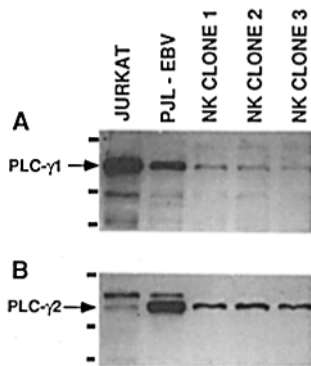
Figure 1. Expression of PLC- \gamma 1 and PLC- \gamma 2 isoforms. Detergent-soluble protein (150 \mu g) from the human leukemic T cell line, Jurkat (lane 1), EBV-transformed human B cells (lane 2), and three different human NK clones (lanes 3–5) were resolved by SDS-PAGE, transferred to nitrocellulose, and probed with a PLC- \gamma 1-specific antiserum (A) as described in Materials and Methods. The same blot was then stripped using a 5 M sodium iodide and 1 mM sodium thiosulphate solution, and reprobed with a PLC- \gamma 2-specific antiserum (B). The molecular mass calibration standards shown on the left are 200, 116, and 96 kD (top to bottom).
