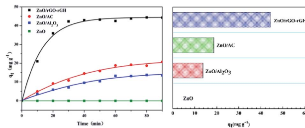
Fig. 6 Adsorption capacities of different composite materials during removing BPA ( C_0 = 10 mg L -1 , [catalyst] = 25 mg).
