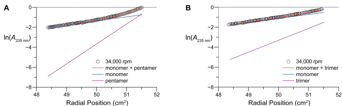
Figure 3. Graphs of analytical ultracentrifugation data obtained at 34000 rpm for host-o and host-r. (A) Data for host-o fitted to a monomer + pentamer mode. (B) Data for host-r fitted to a monomer + trimer mode.
