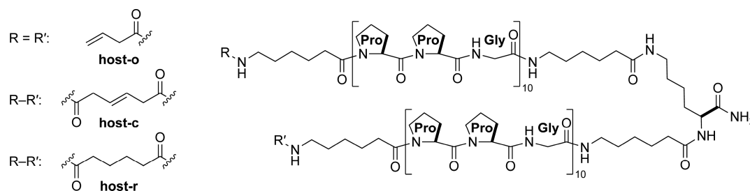
Figure 2. Chemical structures of the open host (host-o), closed host (host-c), and closed, reduced host (host-r). The macrocyclic rings of host-c and host-r contain 221 atoms.
