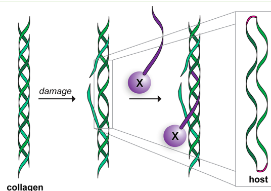
Figure 1. Scheme showing the molecular mimicry of damaged collagen by a cyclic “host” of two parallel collagen strands. A collagen mimetic peptide with a conjugated pendant “X” (purple) is shown annealing to the damaged collagen.
