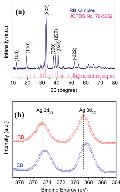
Fig. 2 (a) XRD patterns of RB samples. (b) XPS spectra of the Ag 3d region for RB samples.
