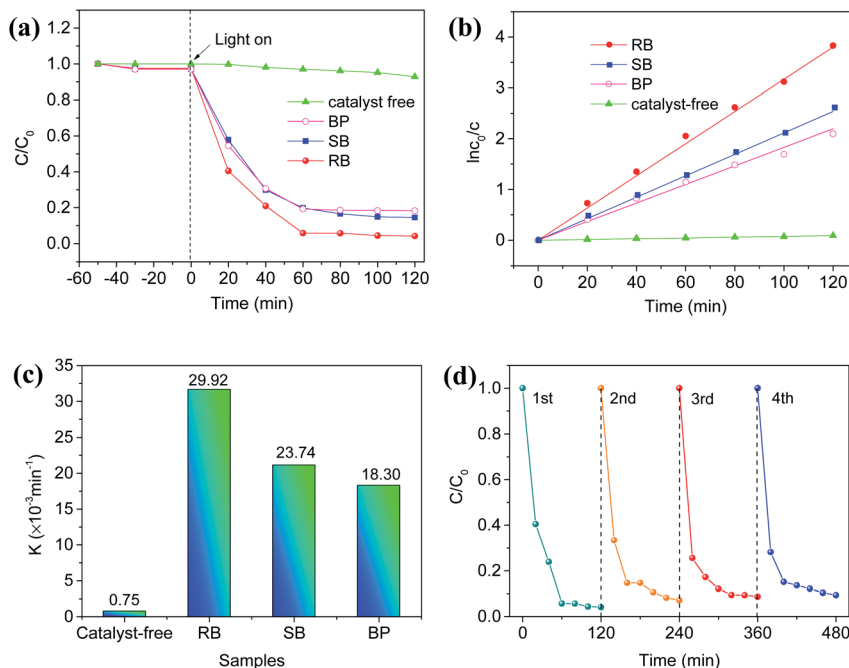
Fig. 5 (a) Photocatalytic degradation of TC over different samples (RB, SB, and BP) in 120 min (the optimum conditions: 50 mg of sample, 20 \text{ mg L}^{-1} of TC solution, pH 9.62, 350 W of the light intensity); (b) the kinetic curves of TC degradation over different samples; (c) the apparent rate constants for TC degradation with different samples; (d) the cyclic degradations of TC over RB samples.
