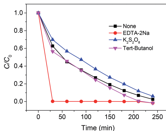
Fig. 7 Trapping experiments for the photoreduction of Cr(vi) over SABC-3 microspheres under visible light irradiation: [\text{Cr}(\text{vi})] = 50 \text{ mg L}^{-1} , m = 40 \text{ g L}^{-1} , \text{pH} = 2.0 .
