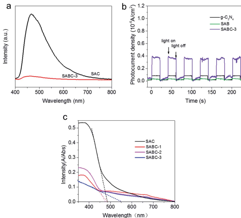
Fig. 4 (a) PL spectra of SAC and SABC-3 microspheres; (b) Photocurrent response density of g- \text{C}_3\text{N}_4 , SAB and SABC-3 microspheres; (c) UV-vis spectra of SAC and SABC microspheres.
