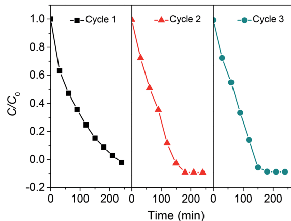
Fig. 6 Recycle experiments of SABC-3 microspheres for photoreduction of Cr(vi): [\text{Cr}(\text{vi})] = 50 \text{ mg L}^{-1} , m = 40 \text{ g L}^{-1} , \text{pH} = 2 .
