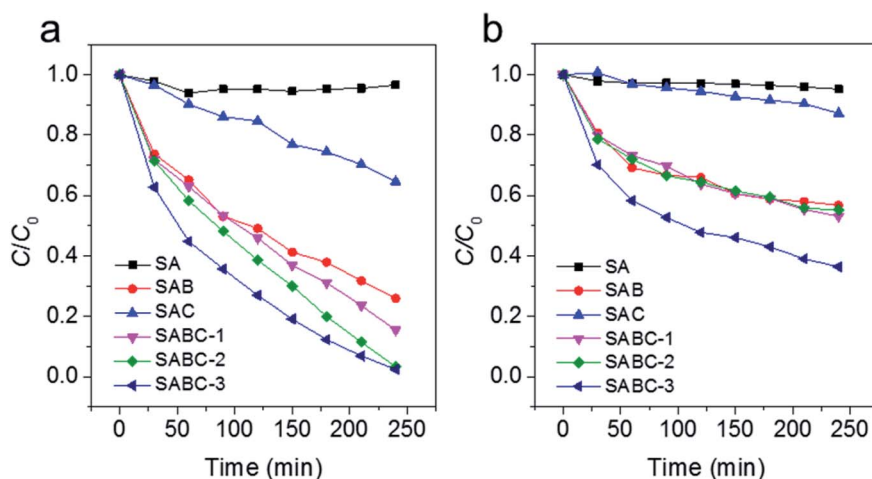
Fig. 5 (a) Photoreduction of Cr(VI) by SA, SAB, SAC and SABC microspheres under visible light irradiation; (b) adsorption of Cr(VI) by SA, SAB, SAC and SABC microspheres: [\text{Cr(VI)}] = 50 \text{ mg L}^{-1} , m = 40 \text{ g L}^{-1} , \text{pH} = 2.0 .
