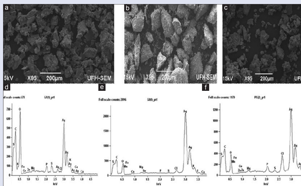
Figure 3: Scanning electron micrographs of nanoparticles derived from (a) garlic, (b) ginger, and (c) cayenne pepper; (d-f) Energy dispersive absorption spectra of silver nanoparticles derived from (d) garlic, (e) ginger, and (f) cayenne pepper
