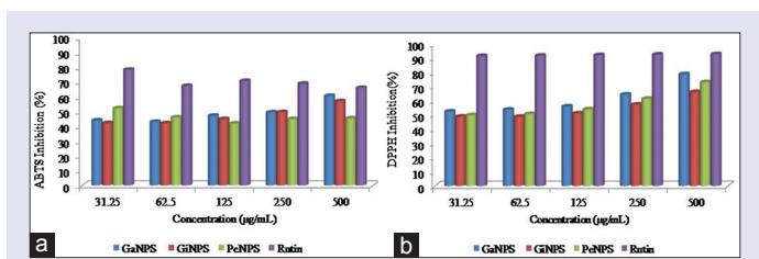
Figure 8: Inhibition of (a) 2,2-Azino-bis(3-ethylbenzthiazoline-6-sulfonic acid) and (b) 1,1-diphenyl-2-picrylhydrazyl radicals by synthesized silver nanoparticles
