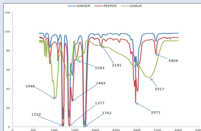
Figure 5: Fourier transform infrared spectra of silver nanoparticles from garlic, ginger, and cayenne pepper
