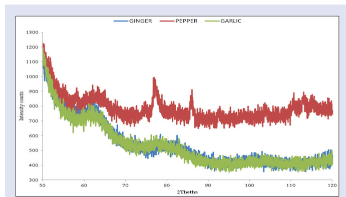
Figure 6: X-ray diffraction pattern of silver nanoparticles from garlic, ginger, and cayenne pepper
