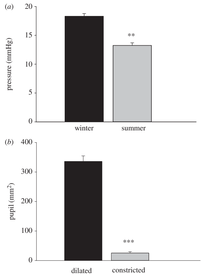
Figure 7. (a) Intra-ocular pressure in eight summer and seven winter eyes (means, s.e.m.). Pressure in winter (18.1 mmHg) was significantly larger than that in summer (13.3 mmHg; **p < 0.01 ). (b) Pupil size in four dilated eyes compared with the fellow eye under bright light. Constricted pupils were 25.3 mm 2 and elongated horizontally. When dilated, they were 336 mm 2 and round ( ***p < 0.001 ).
