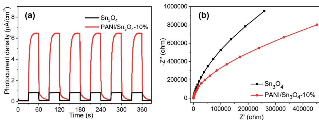
Fig. 8 (a) Instant photo-current density of the synthetic samples under visible light illumination; (b) EIS spectra of Sn 3 O 4 and PANI/Sn 3 O 4 -10% measured at open-circuit voltage.
