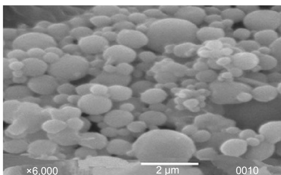
Figure 3 Scanning electron micrograph of chitosan nanoparticles produced using nanoemulsion internal cross-linking technique.
