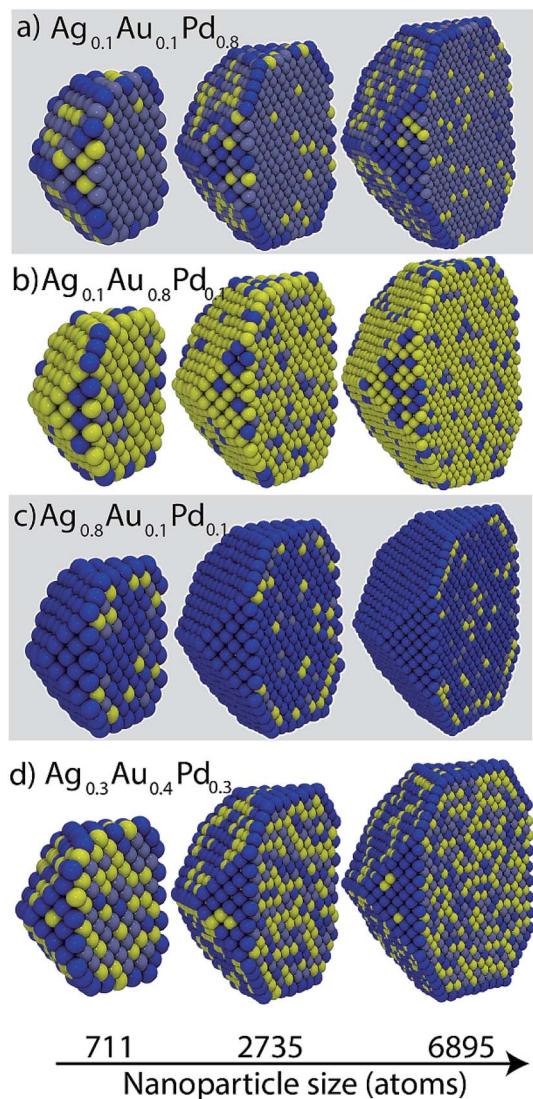
Fig. 8 Cross-sectional views of Ag–Au–Pd NPs. Yellow, dark blue and grayish blue colors denote Au, Ag and Pd, respectively.
