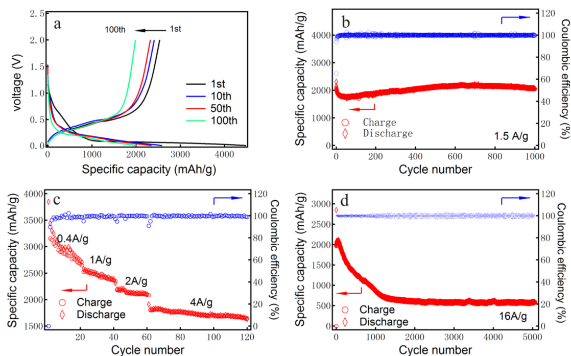
Figure 7. Results of electrochemical performance for 1D-PSiNW anodes. (a) Galvanostatic charge/discharge profiles between 0.01 V and 2.0 V vs. Li/Li + for the first, 10th, 50th, and 100th cycles at a current density of 1.0\text{ A}\cdot\text{g}^{-1} . (b) Cycling performance of the as-prepared 1D-PSiNW anodes at a current density of 1.5\text{ A}\cdot\text{g}^{-1} . (c) Rate performance of 1D-PSiNW anodes at the current density of 0.4/1.0/2.0/4.0\text{ A}\cdot\text{g}^{-1} . (d) Electrochemical performance of 1D-PSiNW anodes with 5000 cycles at a current density of 16.0\text{ A}\cdot\text{g}^{-1} .
