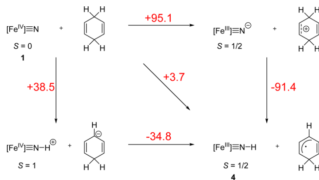
Figure 3. Square scheme for formation of \text{PhB}(\text{MesIm})_3\text{Fe}\equiv\text{NH} 4 by reaction of 1 with 1,4-cyclohexadiene in THF solvent. Lowest energy spin state is shown. Free energy differences are shown in kcal/mol.
