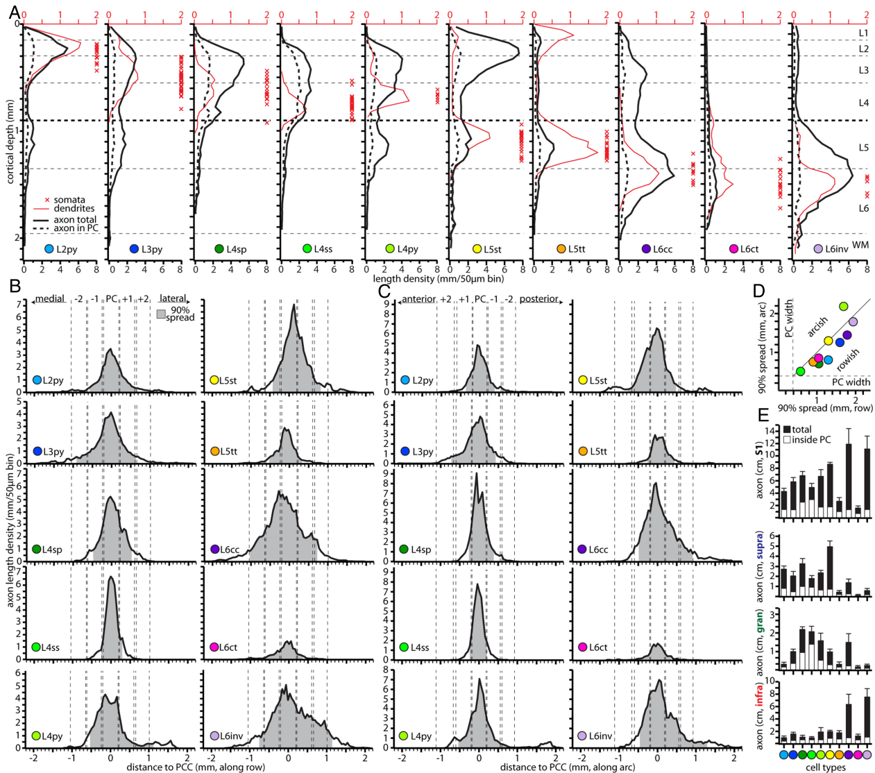
Figure 4. Cell Type-specific vertical and horizontal axon projection patterns. (A) 1D density profiles along vertical cortex axis of dendrites (red) and axons (black), averaged across all neurons assigned to one of the 10 excitatory cell types, respectively. Somata of multiple [supra-]granular cell types intermingled (red "x" denotes the respective soma depths below the pia), but were segregated from infragranular cell types, which also intermingled within and across cytoarchitectonic layers. Dendritic and axonal profiles were cell type-specific, with most axon projecting beyond PC dimensions (inside PC: dashed line profiles; inside vS1: solid line profiles). (B) 1D axon density profiles of the 10 cell types along the row extended in general beyond PC dimensions and even beyond the borders of vS1 (e.g., L6cc). The gray area denotes 90% of the integral below the respective density curves. (C) 1D axon density profiles along the arc (i.e., orthogonal to panel B). (D) Cell type-specific axon extents along the row and arc revealed asymmetric horizontal spreads, with the exception of L4ss and L5st. (E) Quantification of axon projections within (white) and outside (black) the PC reveals cell type- and target layer-specific in/outside PC ratios (from top to bottom: total axon, axon in L1-3, in L4 and L5-6).
