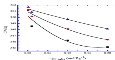
Fig. 17 Plot between CP (K) vs. chloride concentrations for NaCl (■), KCl (●), and \text{NH}_4\text{Cl} (▲), in 0.51 \text{ mmol kg}^{-1} CMT mixed with 6.05, 6.04, and 6.06 \text{ mmol kg}^{-1} TW-80, respectively. This figure is reproduced from ref. 69 with permission from Elsevier, Copyright 2020.
