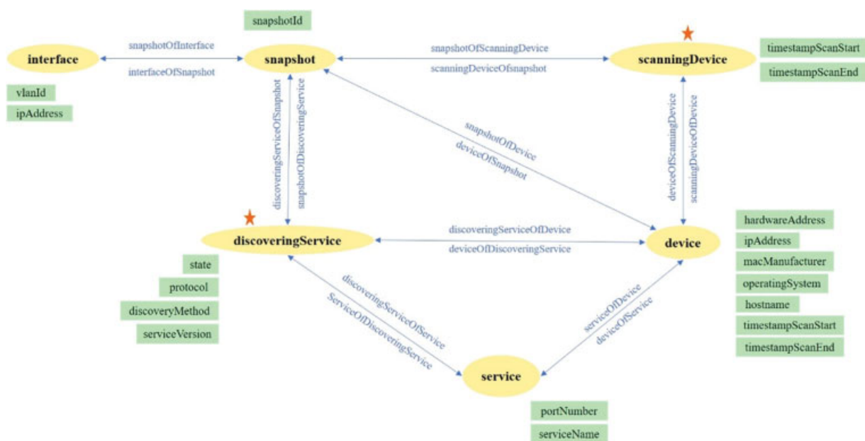
Fig. 1 SDNDL-CAO model. SDNDL-CAO, Software Defined Networking Description Language—CUREX Asset Discovery Tool Ontology.
