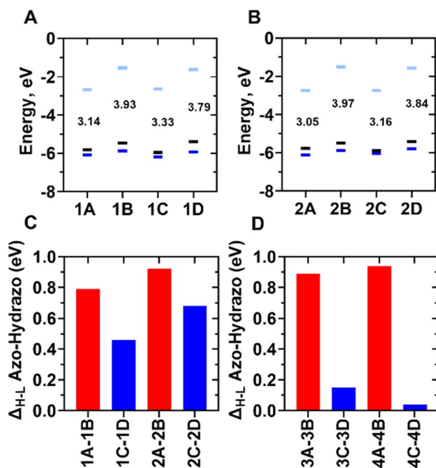
Fig. 2 Frontier molecular orbital energy levels of ortho -TIABP, ortho -TMABP, and their respective hydrazobenzenes in trans and cis conformations. (A) 1A and 1B represent ortho -TIABP and their corresponding hydrazobenzenes in the trans conformation, while 1C and 1D represent ortho -TIABP and their corresponding hydrazobenzenes in the cis conformation. (B) 2A and 2B represent ortho -TMABP and their corresponding hydrazobenzenes in the trans conformation, while 2C and 2D represent ortho -TMABP and their corresponding hydrazobenzenes in the cis conformation. The light blue, black, and blue lines represent the LUMO, HOMO, and HOMO–1, respectively. (C) \Delta_{H-L} gap between ortho -TABP derivatives and their respective hydrazobenzenes in trans (red bars) and cis conformations (blue bars). (D) \Delta_{H-L} gap between ortho -OABP derivatives and their respective hydrazobenzenes in trans (red bars) and cis conformations (blue bars).
