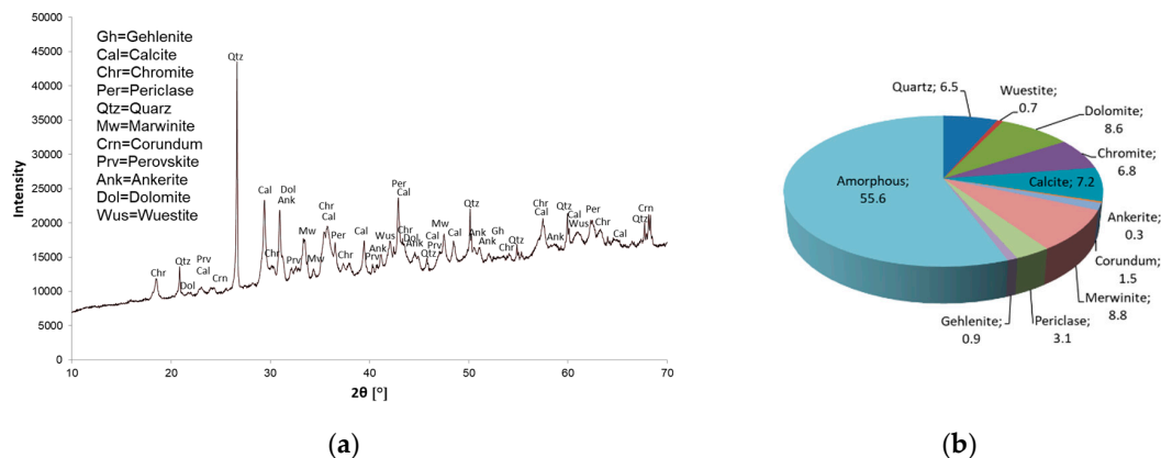
Figure 1. Powder X-Ray diffractogram of Slag A (a) and Rietveld quantification (all in %) of the phases in Slag A (b).
