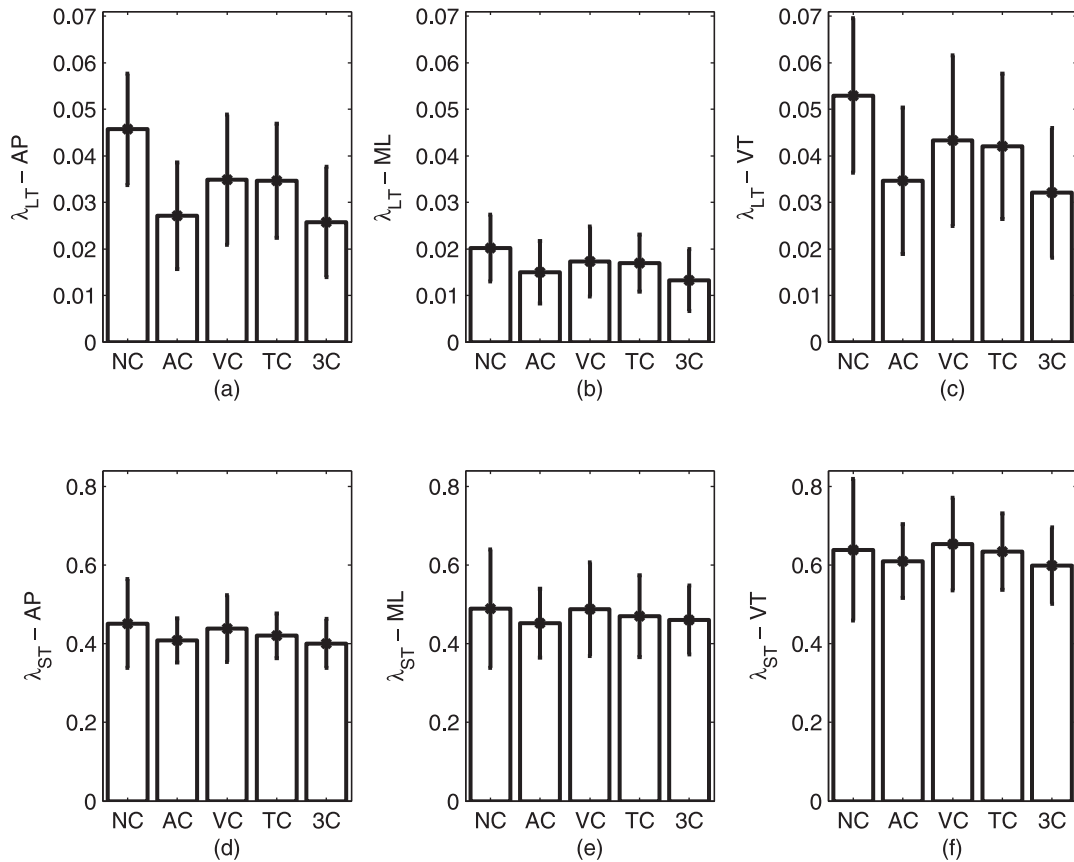
Figure 2. Long and short Lyapunov exponents for the five walking conditions (NC = no cue; AC = auditory cue; VC = visual cue; TC = tactile cue; 3C = three cues). (a) \lambda_{LT} in the AP direction; (b) \lambda_{LT} in the ML direction; (c) \lambda_{LT} in the VT direction; (d) \lambda_{ST} in the AP direction; (e) \lambda_{ST} in the ML direction; and (f) \lambda_{ST} in the VT direction. Error bars denote standard deviation in each case. doi:10.1371/journal.pone.0043104.g002
