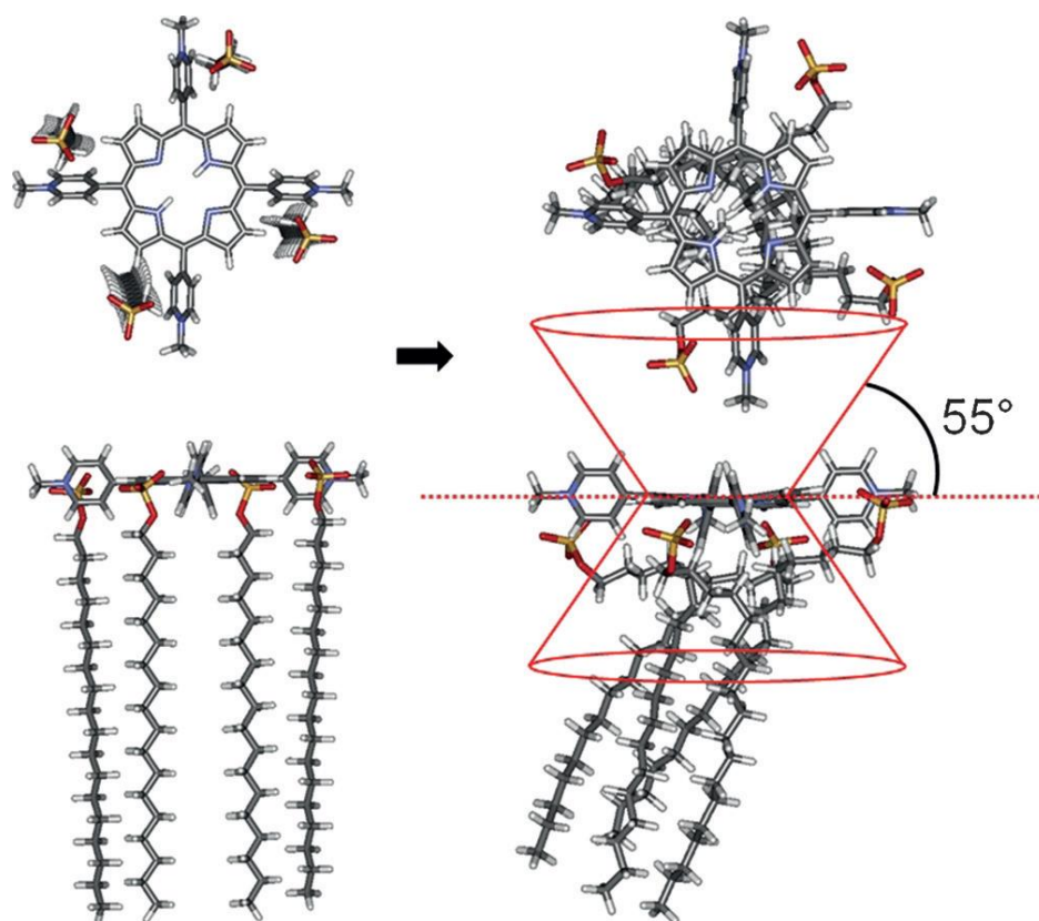
Figure 13. Modeling of the cationic porphyrin- C_{18}OSO_3Na ion pair structure in water reported by Pratiel et al. Reprinted with permission from [62]. Copyright 2015, Wiley.
