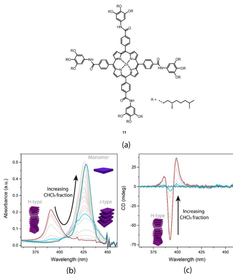
Figure 9. (a) Molecular structure of chiral amide-functionalized Zn porphyrin 11 investigated by Meijer et al. Solvent dependent (b) UV–Vis and (c) CD spectra of 1 \mu\text{M} solutions of 11 , going from methylcyclohexane to solutions with increasing proportions of chloroform. Adapted with permission from [43]. Copyright 2018, American Chemical Society.
