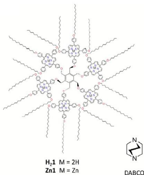
Figure 12. Structure of porphyrin hexamers \text{H}_{21} and \text{Zn}_{11} , and of the bidentate ligand DABCO. Adapted with permission from [61]. Copyright 2018, Royal Society of Chemistry.
