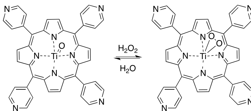
Scheme 3. Schematic drawing for the redox process of the TiOTPyP and its monoperoxo complex of \text{TiO}_2\text{TPyP} [60].
