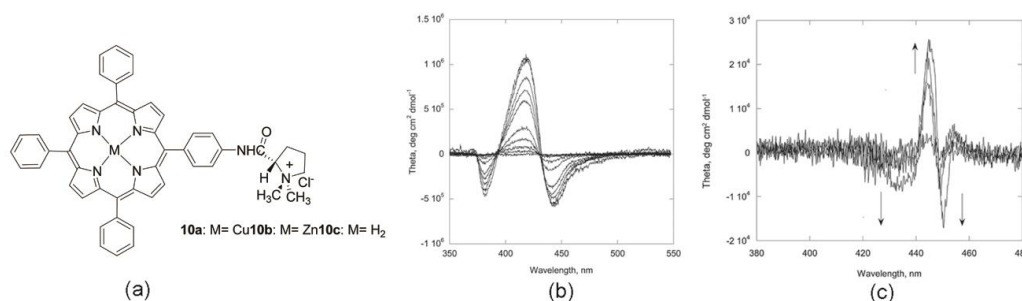
Figure 8. (a) Molecular structure of the conjugated (L)-proline-porphyrin complexes studied by Monti et al. (b) CD variation with time of 10a in EtOH/H 2 O (30%, v:v ) 2.8 \times 10^{-6} M. (c) CD spectral variation with time of 10b in EtOH/H 2 O (25%, v:v ) 4.0 \times 10^{-6} M. Adapted with permission from [42]. Copyright 2019, Royal Society of Chemistry.
