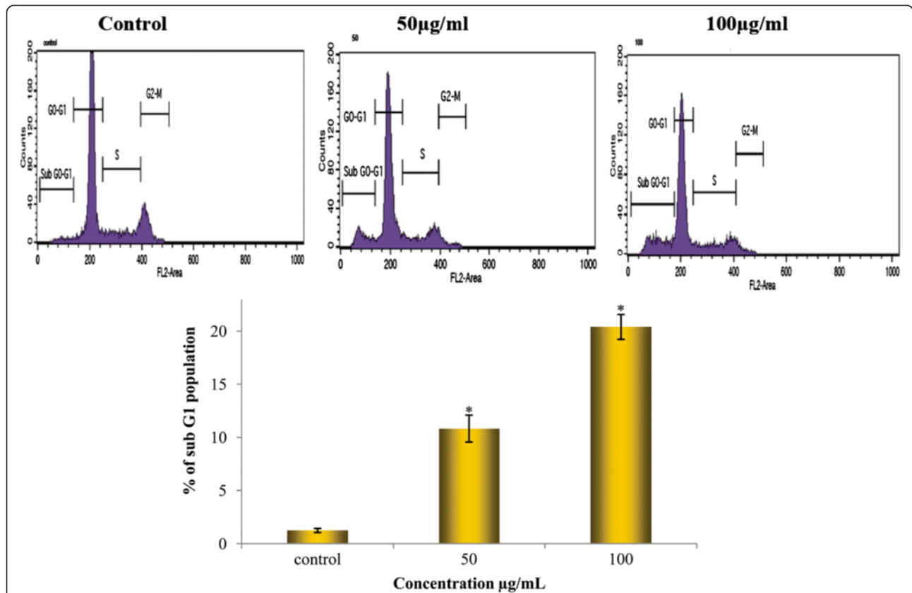
Figure 7 Cell cycle phase analysis by flow cytometry in Huh7 cells treated with TD. The cells were incubated for 48 h with medium alone (control), 50 and 100 µg/ml of TD. A graphic representation of the concentration-dependent increase in the percentage of apoptotic cells following TD treatment. Results are expressed as a percentage of the sub-G1 population obtained from the cells of flow cytometry data of propidium iodide fluorescence as described in Materials and methods, mean ± SD (n =3). Statistical significance *P < 0.05 as compared to the control, in the absence of TD.
