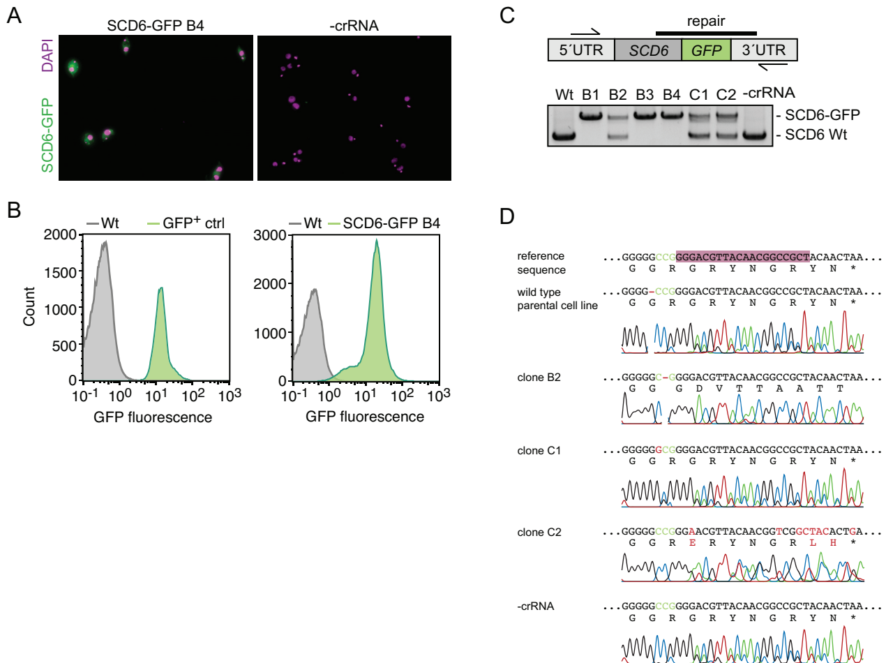
Figure 3. Cas9 allows marker-free genome editing at high efficiency. Unless indicated otherwise, cells were sequentially transfected with the Cas9-episome and the sgRNA-episome(SCD6-GFP.1) and diluted 10 days after transfection. Cells were only analyzed if <20 wells per 96-well plate contained living cells. (A) Fluorescence microscopy analysis of cells transfected with sgRNA-episome(SCD6-GFP.1, clone B4) or a sgRNA-episome lacking a sgRNA (-crRNA). (B) Flow cytometry analysis of edited cells. Left panel: wild type cells (gray) and cells in which SCD6 was GFP-tagged using the pMOT system (55) (green). Right panel: wild type cells (gray) and a representative clone of cells transfected with the sgRNA-episome(SCD6-GFP.1, clone B4). (C) PCR-based analysis of wild type cells, six clones of cells transfected with sgRNA-episome(SCD6-GFP.1) and cells transfected with an sgRNA-episome lacking a sgRNA (-crRNA). Top panel: outline indicating primer binding sites (half arrows). Bottom panel: agarose gel revealing the presence of homozygous (one PCR product) or heterozygous (two PCR products) tagging events. (D) Sanger-sequencing results of the SCD6 gene from wild type cells, the non-edited SCD6 allele of three heterozygous clones and cells transfected with a sgRNA-episome lacking a sgRNA (-crRNA).
