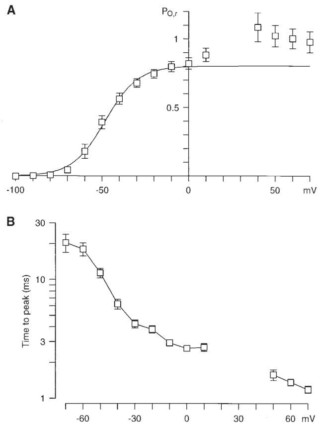
Figure 4. Activation of \alpha 1G channels. (A) Activation curve, from current ratios: the peak current recorded during depolarization directly to the indicated voltage (the protocol of Fig. 1), divided by the instantaneous current recorded after repolarization from a 2-ms step to +60 mV (the protocol of Fig. 3). Data are not shown for voltages near the reversal potential. n = 7 (except n = 6 at +10 mV). The smooth curve is a fit to a Boltzmann functions: V_{1/2} = -48 mV, e-fold for 9.4 mV, amplitude 0.80. (B) Time to peak, for the protocol of Fig. 1, n = 7 .
