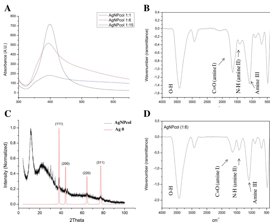
Figure 1 AgNPcol characterization. (A) Absorbance spectra of AgNPcols at three different \text{NaBH}_4 to \text{AgNO}_3 molar ratios; (B) FTIR spectra of collagen; (C) XDR patterns of AgNPcol (1:6 molar ratio); (D) FTIR spectra of AgNPcol (1:6 molar ratio).
