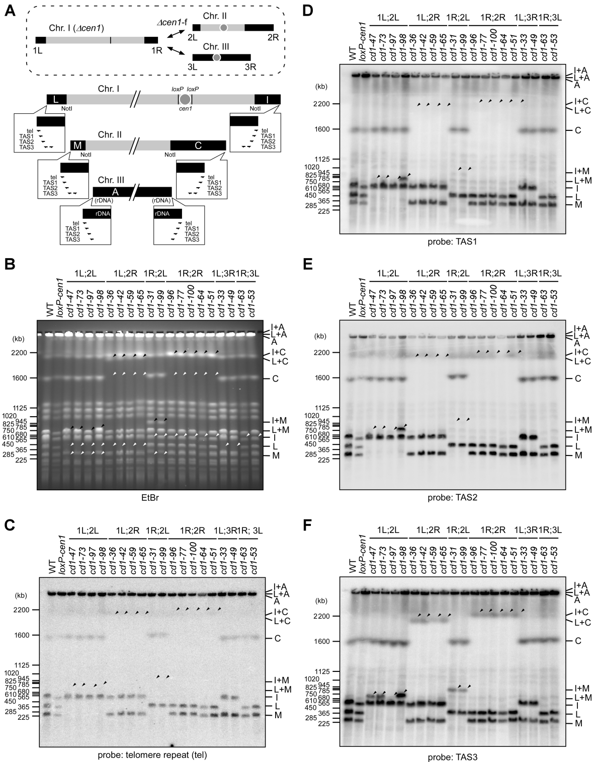
Figure 1. Properties of the fusion ends in the \Delta cen1 survivors. (A) A schematic diagram of fission yeast chromosomes with terminal NotI fragments (black boxes). Their relative positions in the chromosomes are indicated in the upper image representing the \Delta cen1-f rearrangements (dashed circle). The original fragments were detectable by Southern blot probes corresponding to the tel repeat and subtelomere repeats (TAS1, TAS2 and TAS3). The positions and orientations of the repeats are indicated by half arrows in the balloons enlarging the chromosome ends. Nomenclature of the NotI fragments follows previous conventions (64). The cen1 region is flanked by loxP sites to represent the loxP-cen1 construct. (B–F) PFGE analyses of NotI-digested chromosomes of telomere-fusion survivors collected from two individual cen1 deletion experiments. The PFGE samples were subjected to ethidium bromide (EtBr) staining (B) and Southern blotting with the tel (C), TAS1 (D), TAS2 (E) and TAS3 (F) probes. The white arrowheads indicate the disappearance of NotI bands in the survivors due to the fusion rearrangement, and the black arrowheads indicate the newly-generated fusion bands. The identities of the bands with altered migration are indicated at the right-hand side of the gels. A number of the fusion bands failed to hybridize with the tel or subtelomere probes. WT, wild-type; loxP-cen1 , cen1 deletion strain.
