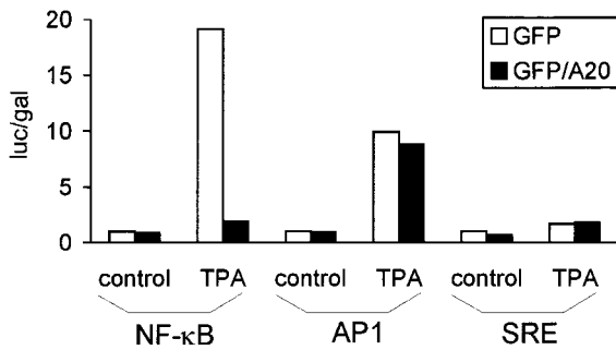
Figure 5. Effect of A20 on TPA-induced activation of gene expression mediated by NF- \kappa B, AP1, or SRE. 293T cells were transfected with 100 ng pUT651 and 100 ng NFconluc, pAP1-luc, or pSRE-luc, in combination with 100 ng pCAGGS-GFP or pCAGGS-GFP/A20. Cells were either left untreated or treated with 200 ng/ml TPA for 6 h. Cells were analyzed for luciferase expression as described in Materials and Methods. Data from a representative experiment (total number of experiments, 2) are expressed as the mean ( n = 3 ) with SD < 10%.
