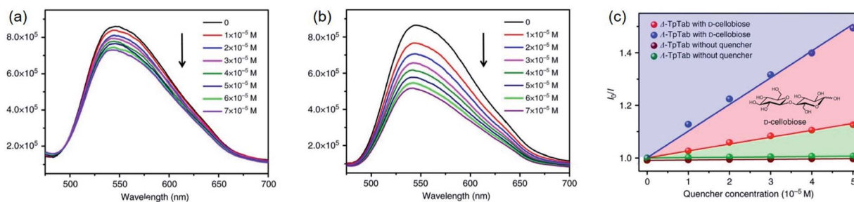
Fig. 24 (a and b) The fluorescence emission spectra of the (\Lambda)/(\Delta) -TpTab COF with increasing concentration of the D-cellobiose quencher. (c) SV plots of the fluorescence emissions of the (\Lambda)/(\Delta) -TpTab COF quenched by D-cellobiose. Adapted from ref. 30. Copyright 2018 Nature Research.
