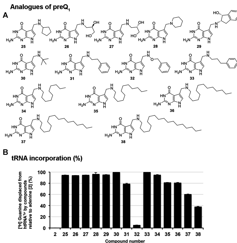
Figure 3. Substrate scope: influence of substitution of the methylene amine of preQ 1 . (A) Derivatives of preQ 1 with substitutions at the methylene amine. (B) Nucleobases (50 \mu M) were assessed for their ability to displace [ 3 H] Guanine from pre-labeled tRNA Tyr (10 \mu M) catalyzed by the QTRT enzyme (100 nM). Data are mean \pm SD ( n=3 ). Representative of two independent experiments.
