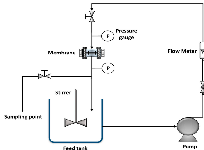
Figure 2. Schematic diagram of the flow loop system.
