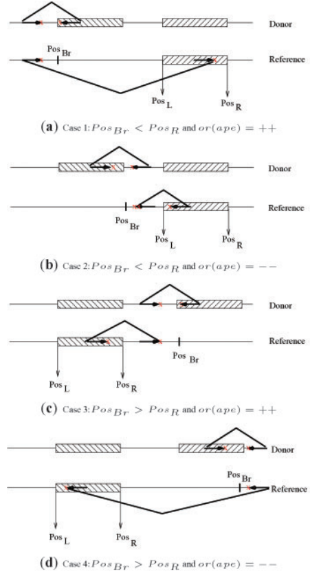
Fig. 3. The set of conditions for each case that suggests a copy event in which the transposed segment is copied in inverted orientation (Class II). (a) Case 1: Pos_{Br} < Pos_R and or(ape) = ++ , (b) Case 2: Pos_{Br} < Pos_R and or(ape) = -- , (c) Case 3: Pos_{Br} > Pos_R and or(ape) = ++ , (d) Case 4: Pos_{Br} > Pos_R and or(ape) = -- .
