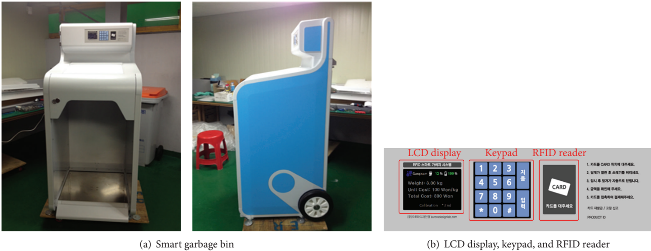
FIGURE 9: (a) Smart garbage bin and (b) LCD display, keypad, and RFID reader.
