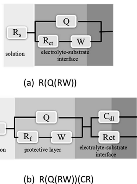
Fig. 3 Electrochemical equivalent circuits simulated for the impedance of bare copper (a), and 4-PPM modified copper (b).
