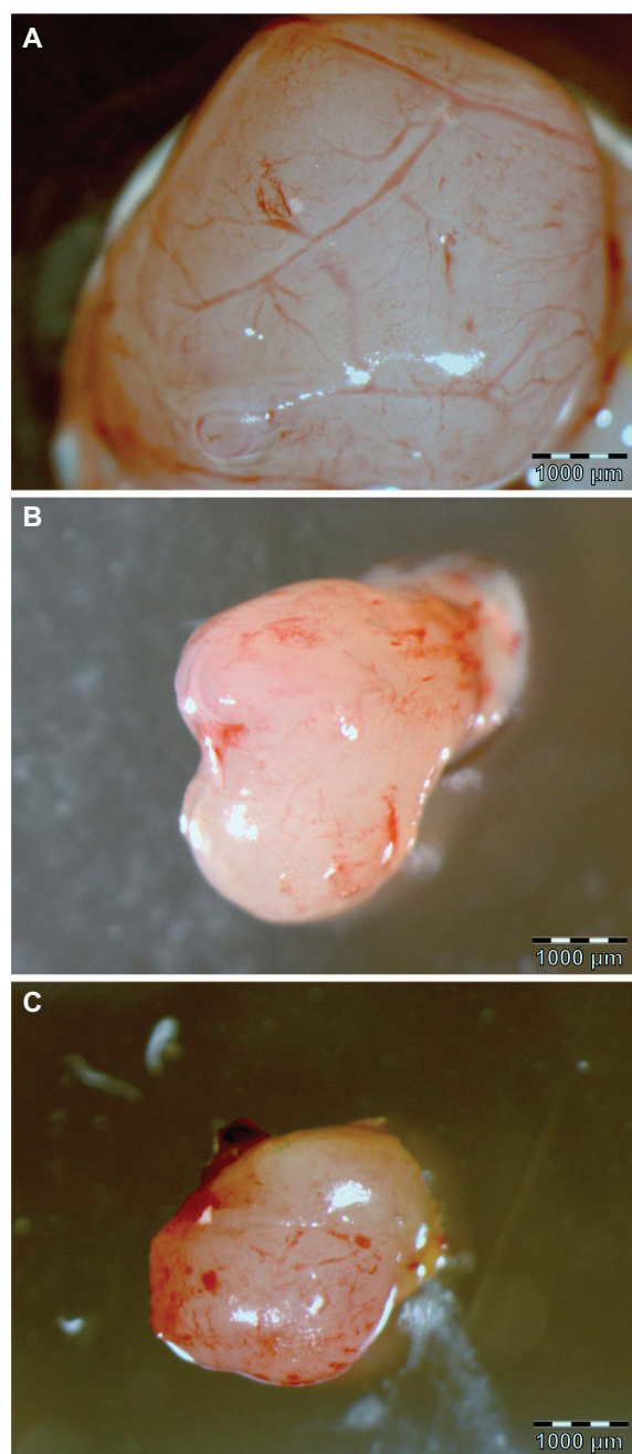
Figure 4 Images of a glioblastoma multiforme tumor cultured on chorioallantoic membrane: (A) control group, (B) ultradispersed detonation diamond group, and (C) microwave-radiofrequency group. Note: Scale bar: 1000 µm.
