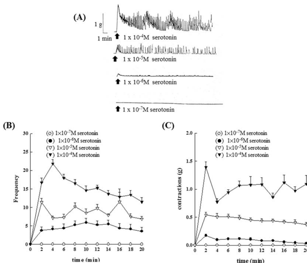
Fig. 6. Effects of different concentrations of 5-HT on the isolated epididymal vas deferens of rats. 5-HT ( 1 \times 10^{-7} \text{M} – 1 \times 10^{-4} \text{M} ) showed a dose-dependent increase in the contraction amplitude (6A), frequency (6B) and the contraction force (6C) of the rat epididymal vas deferens. The maximum contraction tension was 0.17 \pm 0.03 , 0.54 \pm 0.05 , and 1.39 \pm 0.09 , respectively.
