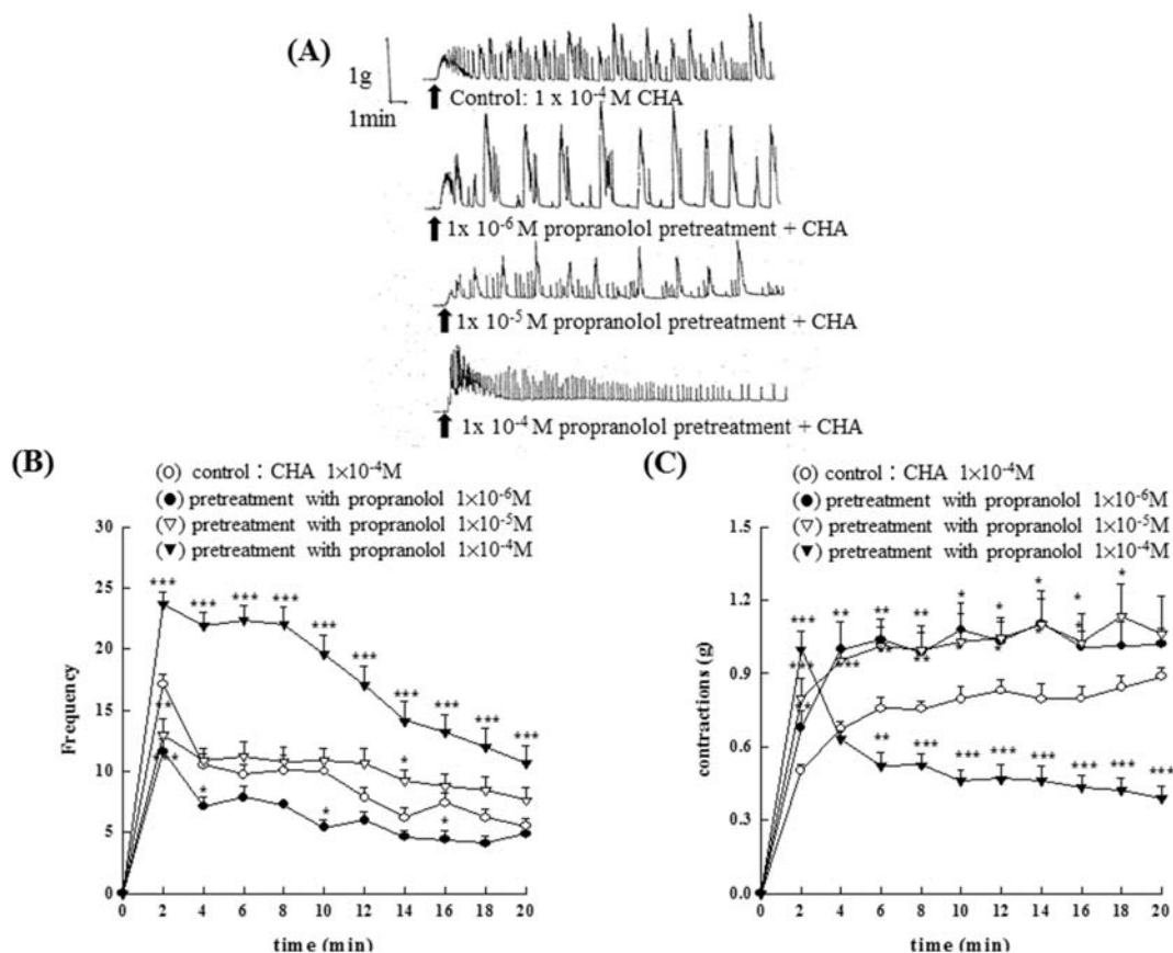
Fig. 5. Effects of 5-HT 1 serotonergic antagonists on the contraction of the isolated epididymal vas deferens of rats induced by CHA. With the increase of the time, propranolol ( 1 \times 10^{-5} M and 1 \times 10^{-6} M) enhances the CHA-induced contraction of the vas deferens. Fig. 5A represented the contraction trace of isolated rat epididymal vas deferens, the frequency change (Fig. 5B), and the contraction force (g) change in CHA and propranolol pretreatment in Fig. 5C. Propranolol at the concentration of 1 \times 10^{-4} M showed a suppression effect on CHA-induced contraction ( P < 0.01 ) and the frequency of contraction increased significantly ( P < 0.01 ).
