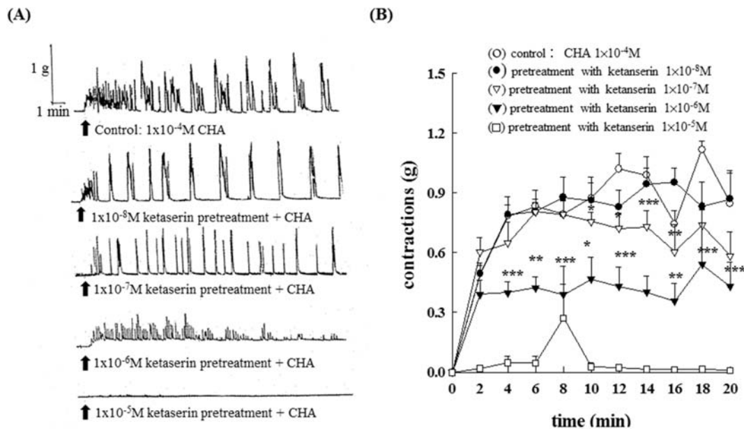
Fig. 4. Effects of 5-HT 2 /5-HT 1C serotonergic antagonist, ketanserin, on the CHA-induced contraction of the isolated epididymal vas deferens of rats. Fig. 4A represented the contraction trace of isolated rat epididymal vas deferens and the contraction force (g) change in CHA and ketanserin pretreatment in Fig. 4B ( P < 0.05 ~ P < 0.001 ). The CHA-induced contraction of epididymal vas deferens was completely inhibited by ketanserin at the concentration of 1 \times 10^{-5} M .
