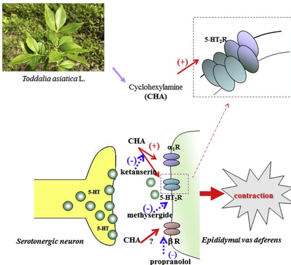
Fig.10. Proposed action mechanism of cyclohexylamine (CHA)-induced contraction of epididymal vas deferens of rat. CHA induced contraction on the isolated rat epididymal vas deferens may be partially mediated by serotonergic neuron.
