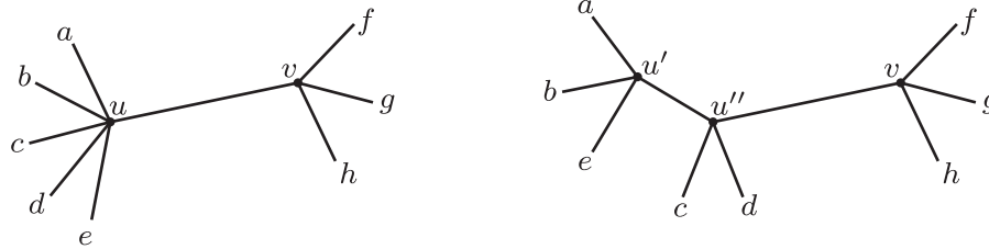
FIGURE 1. The tree on the right resolves the tree on the left by the addition of an edge ( u', u'' ) to resolve vertex u . The tree on the right displays any character \chi that assigns taxa a, b, e one state and c, d, f, g, h a second state, so \chi is compatible with this tree as well as the tree on the left (even though that tree does not display \chi ).
