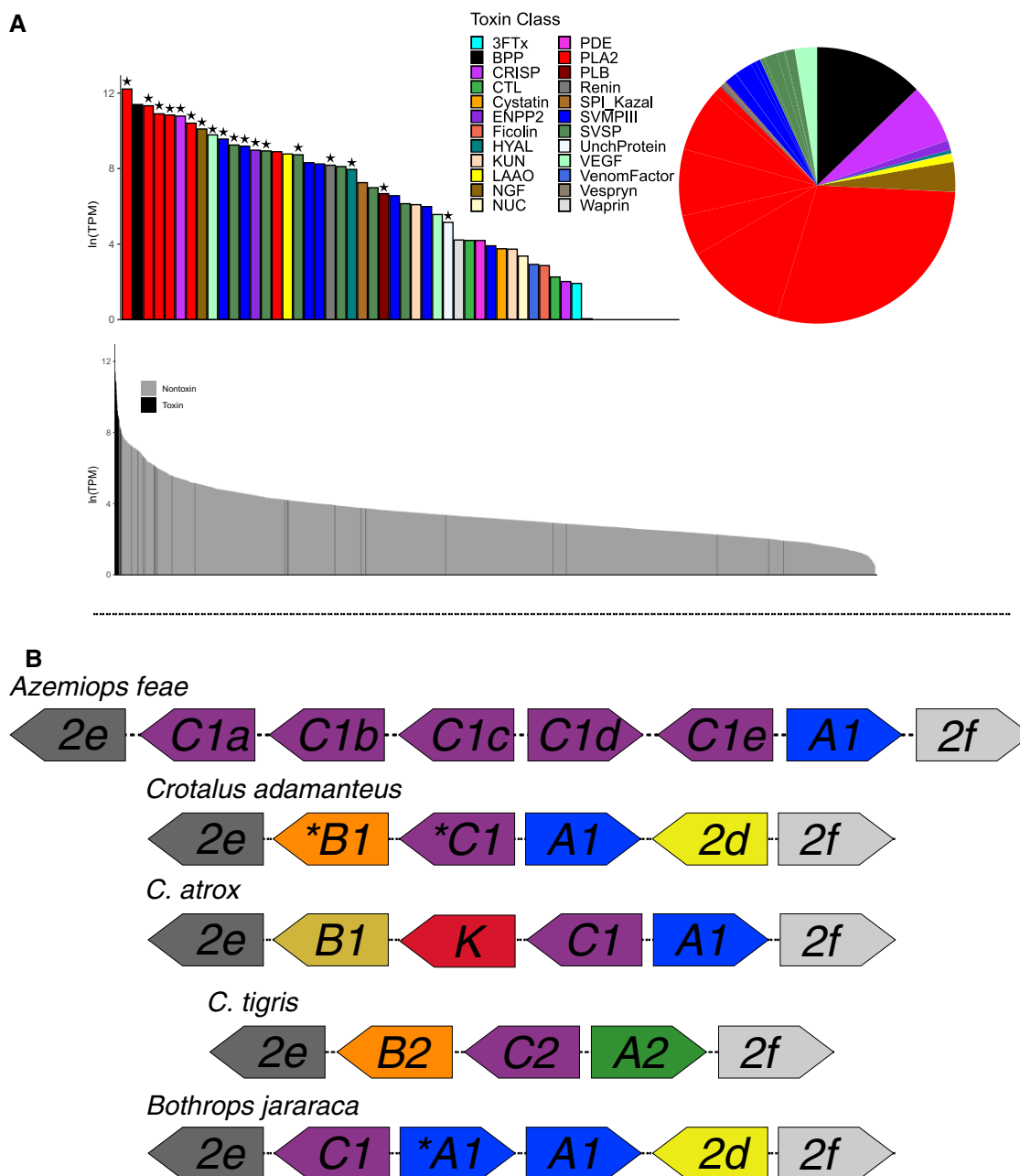
Fig. 2. —(A) The expression of each recovered toxin transcript plotted as \ln(\text{TPM}) and colored by toxin class, a "*" above a toxin indicates verification via proteomics. The pie-chart represents the proportion of toxin gene expression by class, demonstrating the large proportion of \text{PLA}_2 gene expression within A. feae . Gray and black histogram represents total toxin and nontoxin gene expression within the venom gland; (B) schematic architecture of the \text{PLA}_2 gene family in A. feae compared with members of the Crotalinae ( Crotalus species and Bothrops jararaca ) demonstrating the shared architecture of \text{PLA}_2 -gC::gA1 across taxa. This also illustrates the numerous hypothesized independent duplications of \text{PLA}_2 -gCs within A. feae and gene losses in members of the Viperidae. Toxin abbreviations: three-finger toxin (3FTx), Bradykinin-potentiating peptides (BPP), cysteine-rich secretory proteins (CRISP), C-type lectins (CTL), ectonucleotide pyrophosphatase/phosphodiesterase 2 (ENPP2), hyaluronidase (HYAL), Kunitz-type proteinase inhibitor (KUN), L-amino acid oxidase (LAAO), nerve growth factor (NGF), Ecto 5' nucleotidase (NUC), phosphodiesterase (PDE), phospholipase \text{A}_2 ( \text{PLA}_2 ), phospholipase B (PLB), Kazal-type serine protease inhibitor (SPI_Kazal), snake venom metalloproteinase (SVMP), snake-venom serine protease (SVSP), uncharacterized protein (UnchProtein), and vascular endothelial growth factor (VEGF).
