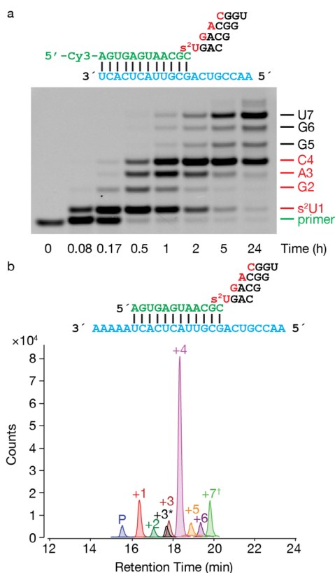
Figure 3. Efficient one-pot extension of primers by four nucleotides. (a) Electrophoretogram of extension products after different reaction times, as assayed by PAGE. Positions of primer and +1 to +7 products are indicated. Reaction conditions: 1.2 \mu M primer (green), 1.5 \mu M template (cyan), 200 mM HEPES pH 8.0, 50 mM MgCl_2 , 0.5 mM trimer (black), and 10 mM monomer (red). (b) Overlay of extracted ion chromatograms of residual primer (P) and extension products after 1 day (+1 to +7) observed by LC-MS. Observed ions for the peak labeled +3* are consistent with a product having misincorporated s^2U in place of A at the +3 position. Observed ions for the peak +7 † are consistent with either the correct +7 product or an alternative double mutant product (see Table S1).
