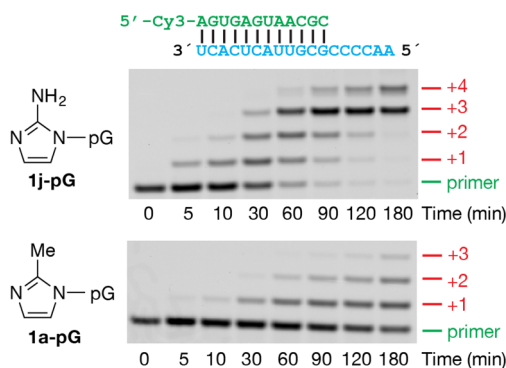
Figure 2. Efficient nonenzymatic RNA copying using phosphoroimidazolides with 2-AI leaving group. The time course of primer extension reaction using phosphoroimidazolides 1j-pG and 1a-pG were assayed using polyacrylamide gel electrophoresis (PAGE). Positions of primer and +1 to +4 products are indicated. Reaction conditions as described in Figure 1.
