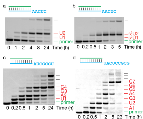
Figure 4. Efficient one-pot nonenzymatic copying of various short RNA templates. (a) Copying AA dinucleotide templates using 2-AI activated U monomers and trimers. (b) Copying AA dinucleotide templates using 2-AI activated s^2U monomers and trimers. (c) Extending primers by UAGC using 2-AI activated A, C, G, and U monomers and trimers. (d) Extending primers by the sequence AUGAGGC using 2-AI activated A, C, G, and U monomers and trimers. The extension products were assayed by PAGE. Positions of primers and extended products are indicated. Reaction conditions as described in Figure 3.
