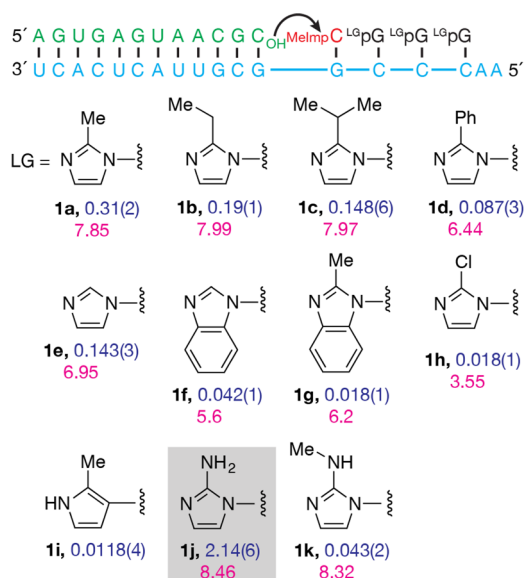
Figure 1. Development of 2-aminoimidazole as a superior leaving group for nonenzymatic primer extension. Top row: the template (cyan)-dependent reaction of 2-MI activated C monomers (red) with the primer (green) was used to probe the effect of adjacent leaving groups (LG, black) on the reaction rate. Curved arrow indicates the site of reaction. Varying the leaving group (1a–1k) influenced the rates by up to 200 times, with 2-aminoimidazole (1j) giving the fastest rate. Reaction conditions: 1.5 \mu M primer, 5 \mu M template, 200 mM HEPES pH 8.0, 50 mM MgCl_2 , and 20 mM monomers. All experiments were performed in triplicate. Blue: mean observed rate in h^{-1} ; standard error of the mean (s.e.m.) in the last digit is shown in parentheses. Magenta: pK_a of the leaving group.
