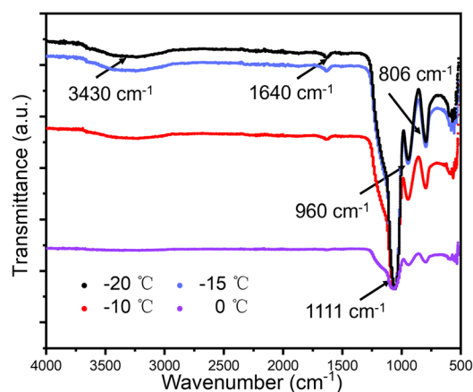
Fig. 8 FT-IR diagram of silica spheres synthesized with the System B by the pre-reaction and low-temperature strategy: the pre-reaction time was 1 min, the cooling temperatures were 0\text{ }^{\circ}\text{C} , -10\text{ }^{\circ}\text{C} , -15\text{ }^{\circ}\text{C} , and -20\text{ }^{\circ}\text{C} , respectively.
