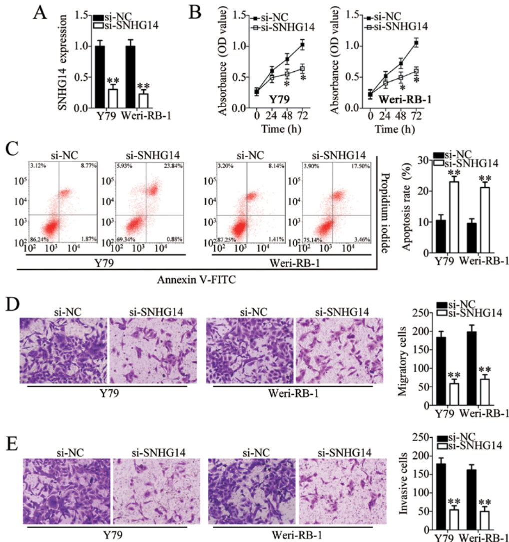
Figure 2. Silencing of SNHG14 represses the proliferation, migration, and facilitates the apoptosis of Y79 and Weri-RB-1 cells. (A) Y79 and Weri-RB-1 cells were transfected with either si-SNHG14 or si-NC. Expression of SNHG14 was analyzed at 48 h post-transfection. **P<0.01 vs. the si-NC group. (B) Proliferation of SNHG14 -deficient Y79 and Weri-RB-1 cells was quantitated in the Cell Counting Kit-8 assay. *P<0.05 vs. the si-NC group. (C) Flow cytometry was utilized to measure the apoptotic rates of Y79 and Weri-RB-1 cells following either si-SNHG14 or si-NC transfection. **P<0.01 vs. the si-NC group. (D and E) The levels of migration and invasion in the SNHG14 knockdown Y79 and Weri-RB-1 cells were assessed using (D) Transwell migration and (E) invasion assays. Magnification, x200 magnification. **P<0.01 vs. the si-NC group. SNHG14 , small nucleolar RNA host gene 14; si, small interfering RNA; NC, negative control; FITC, fluorescein isothiocyanate.
