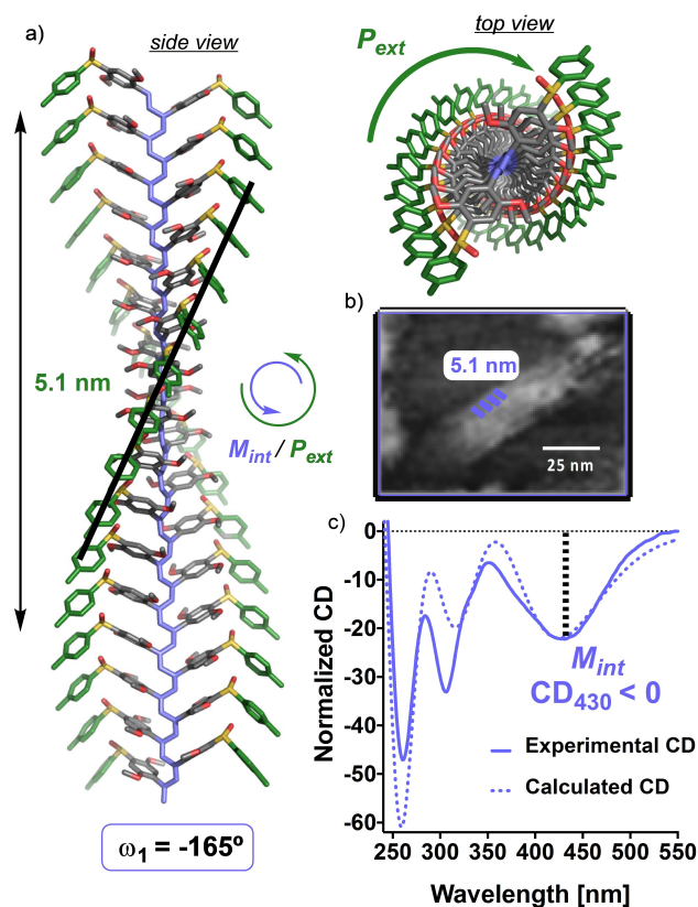
Figure 3. a) 3D structure adopted by poly-( R )-1 in \text{CHCl}_3 . b) AFM image of a 2D crystal of poly-( R )-1 prepared in \text{CHCl}_3 . c) Theoretical and experimental ECD spectra of poly-( R )-1 (normalized at 430 nm). [poly-( R )-1] = 0.3 mg mL -1 .
