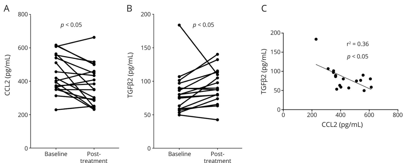
Figure 3 Decreased CCL2 and increased TGF- \beta 2 in CSF following IT-MSC-NP treatment
